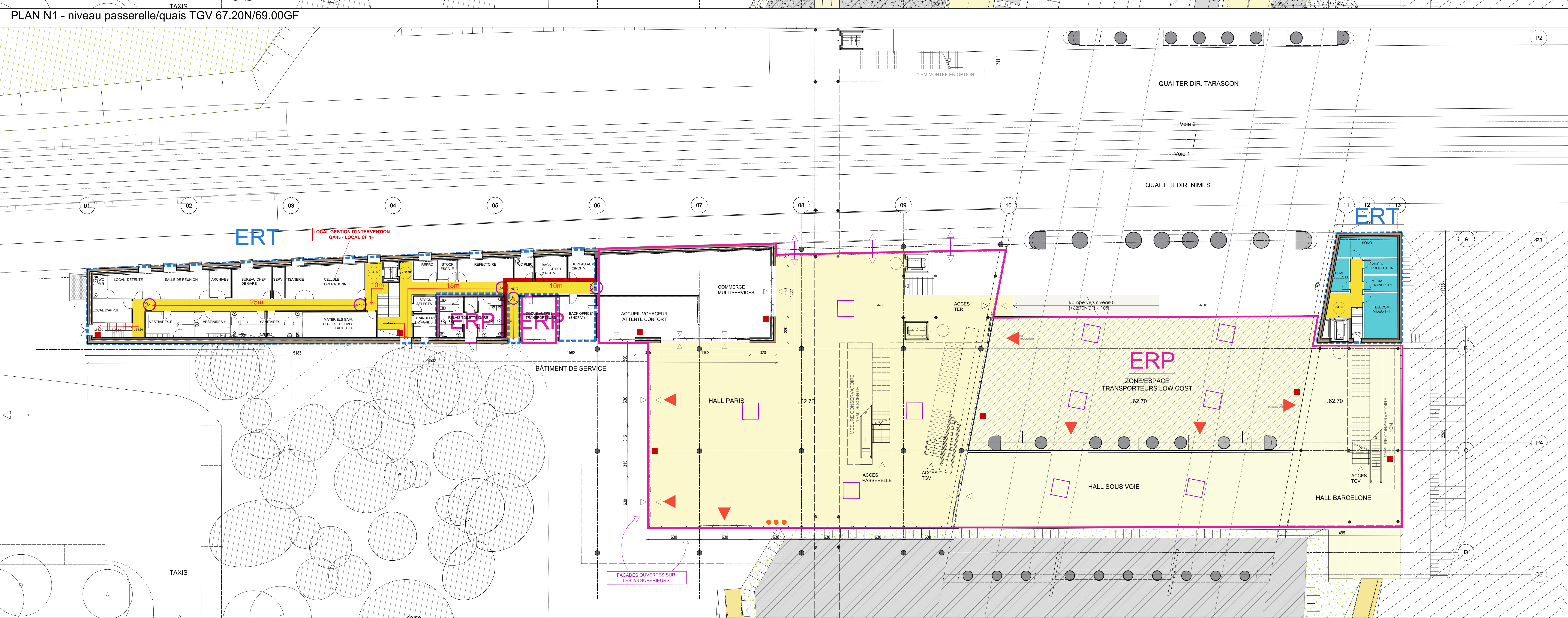
PLAN REZ DE PARVIS 62.70NGF
